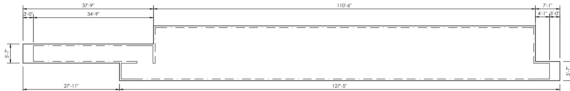
FOUNDATION LAYOUT SCALE: 1/8"=1'-0"
